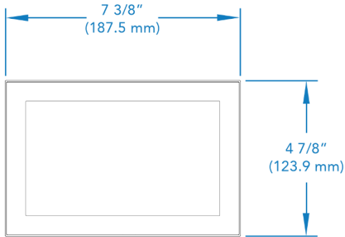
MSD-701 (Front View)
