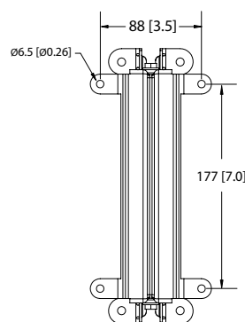
Wall-Mount Section
